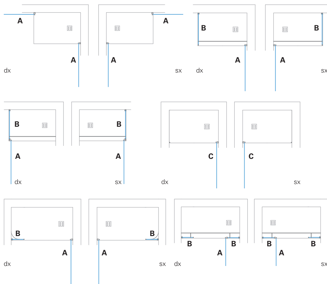
Cerniera profilo / Profile hinge
