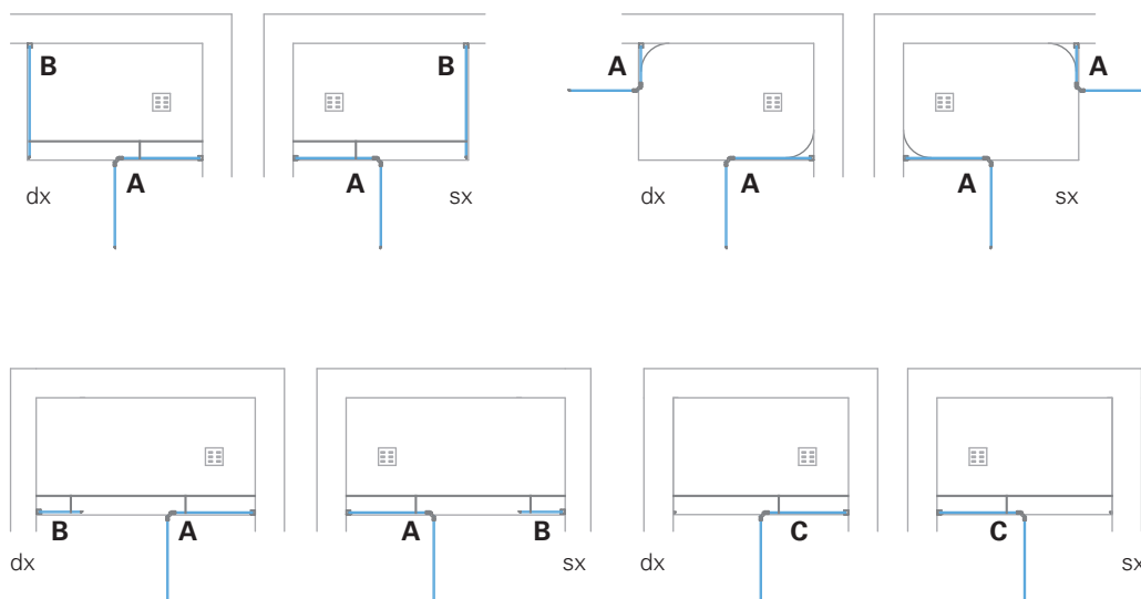
Cerniera CER005 / Hinge CER005
